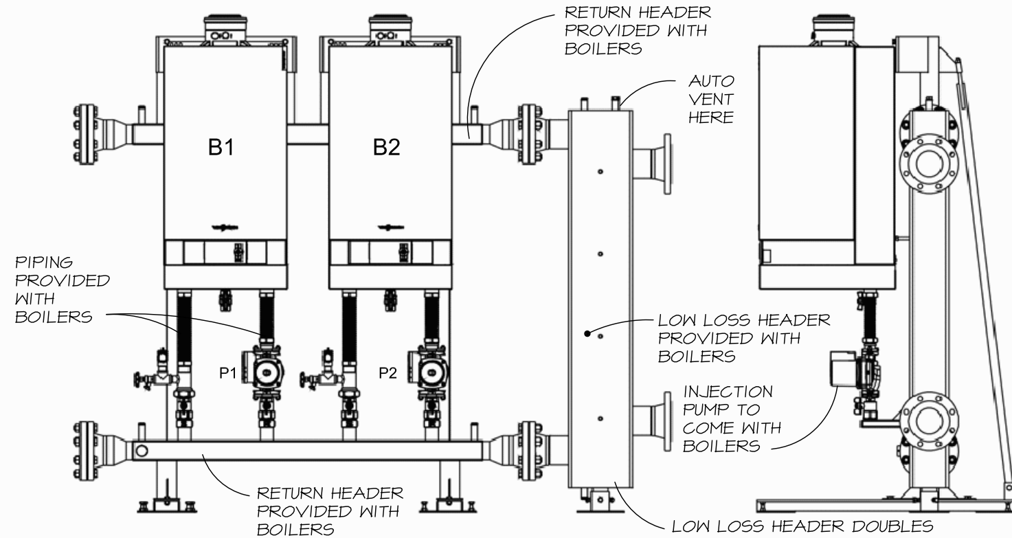
1 BOILER PIPING DIAGRAM NO SCALE
