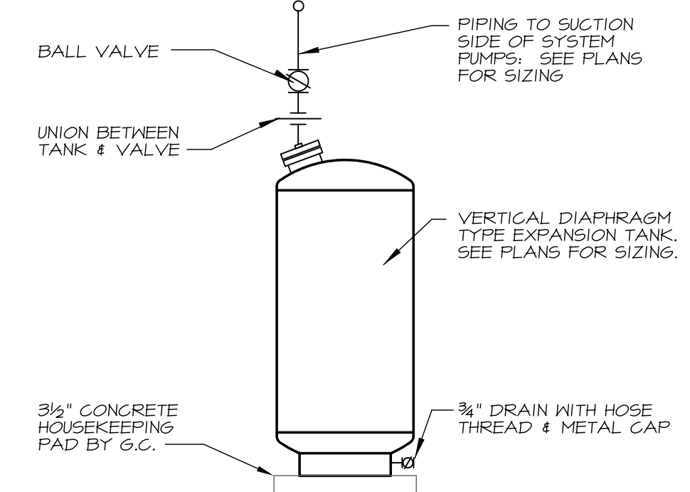
5 DIAPHRAGM TYPE EXPANSION TANK NO SCALE
