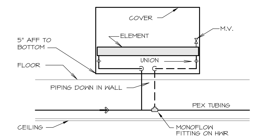
11 UPFEED CONVECTOR NO SCALE
