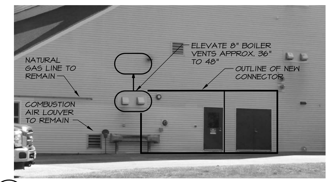
14 EXISTING BUILDING AT CONNECTOR NO SCALE
