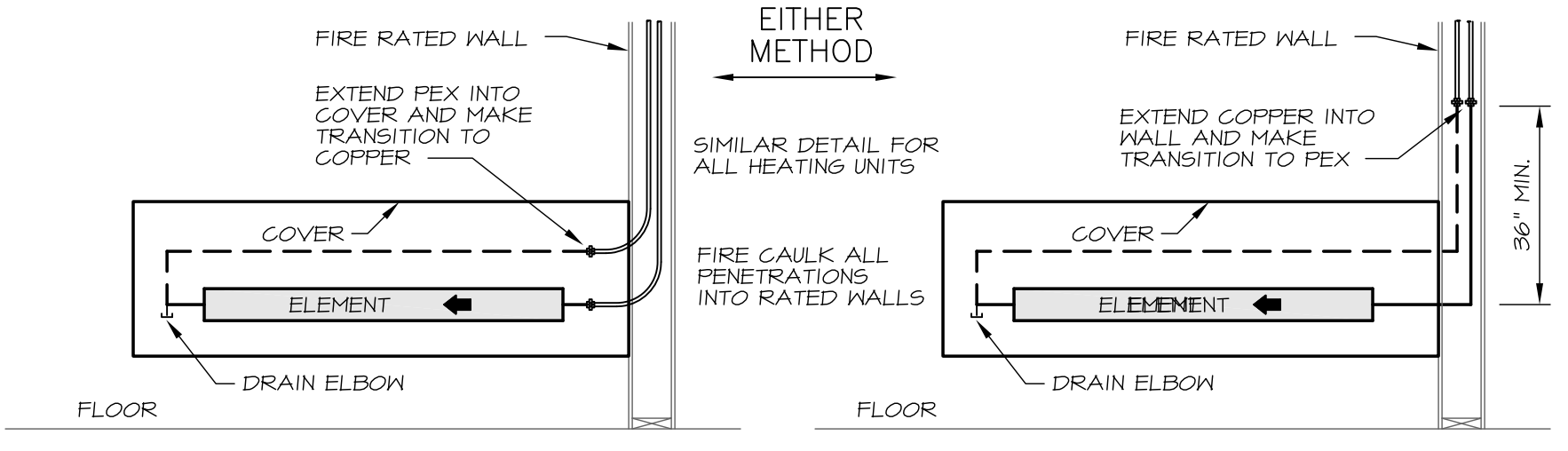
6 DOWNFEED PIPING WITH PIPING IN RATED WALLS NO SCALE
