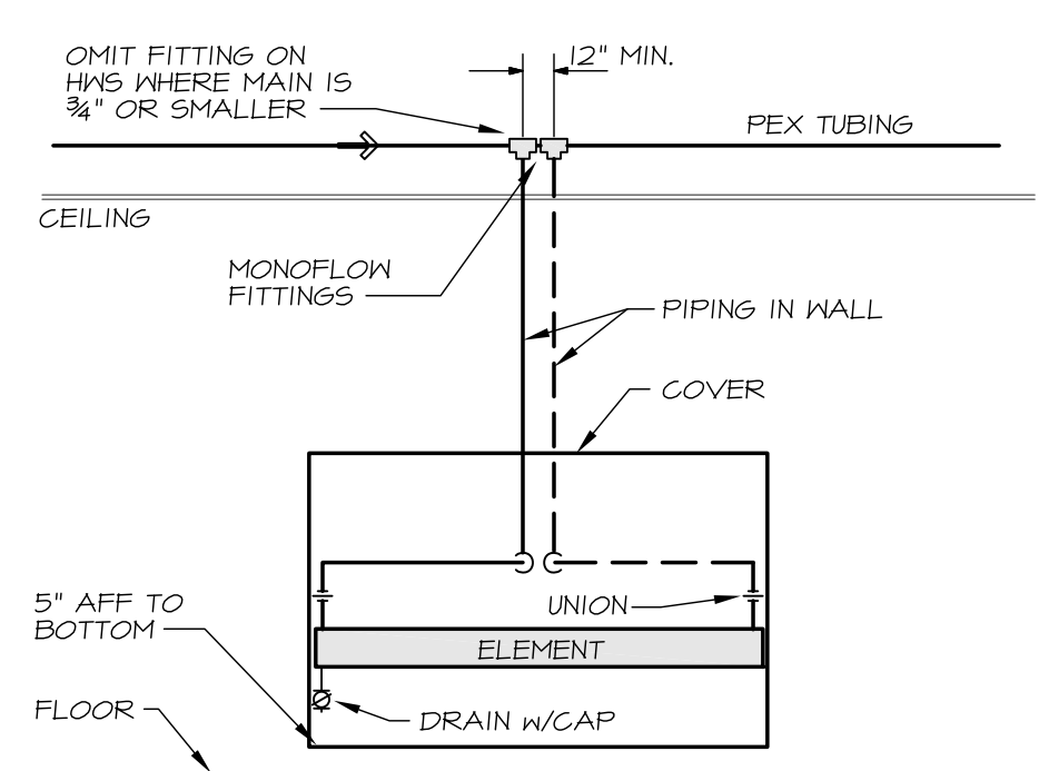
12 DOWNFEED CONVECTOR NO SCALE
