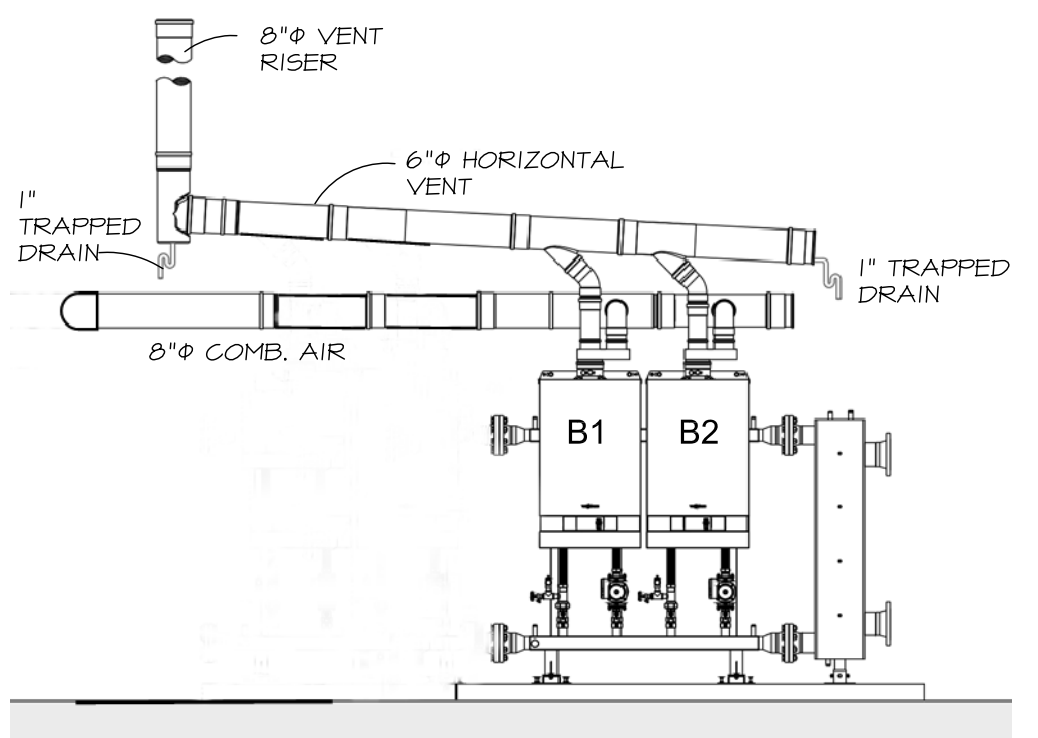
3 BOILER VENTING DIAGRAM NO SCALE
