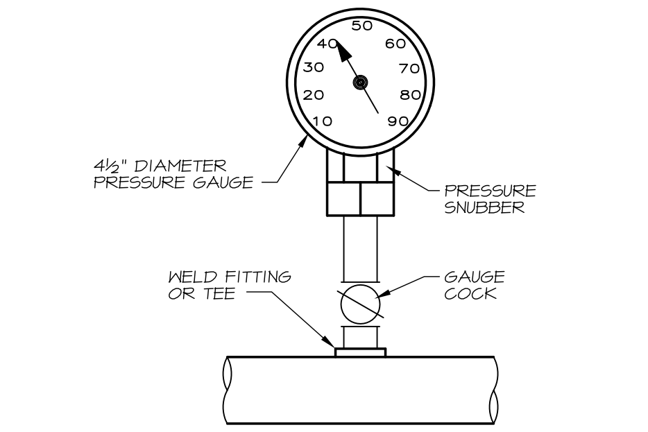
8 WATER PRESSURE GAUGE NO SCALE
