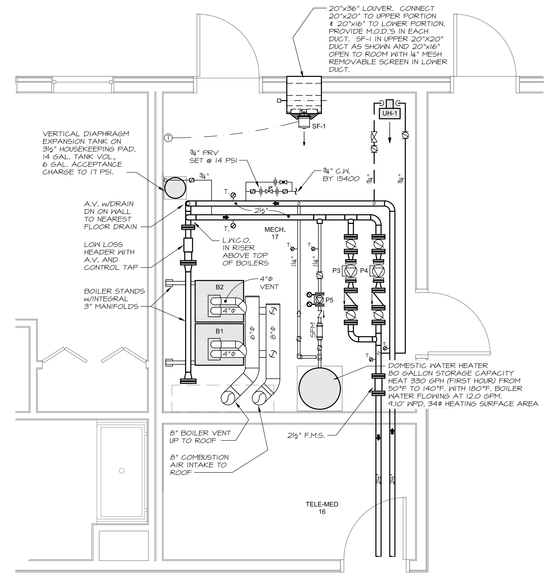
13 MECHANICAL ROOM PLAN SCALE: 3/8" = 1'-0"
