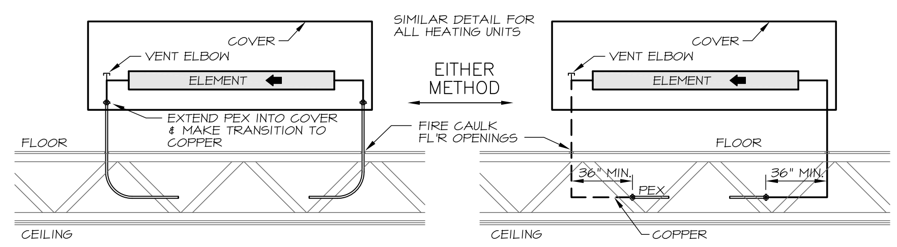
7 UPFEED PIPING THROUGH RATED FLOOR/CEILING NO SCALE
