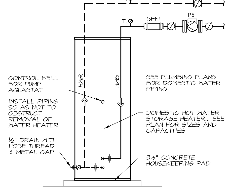
4 STORAGE WATER HEATER DETAIL NO SCALE
