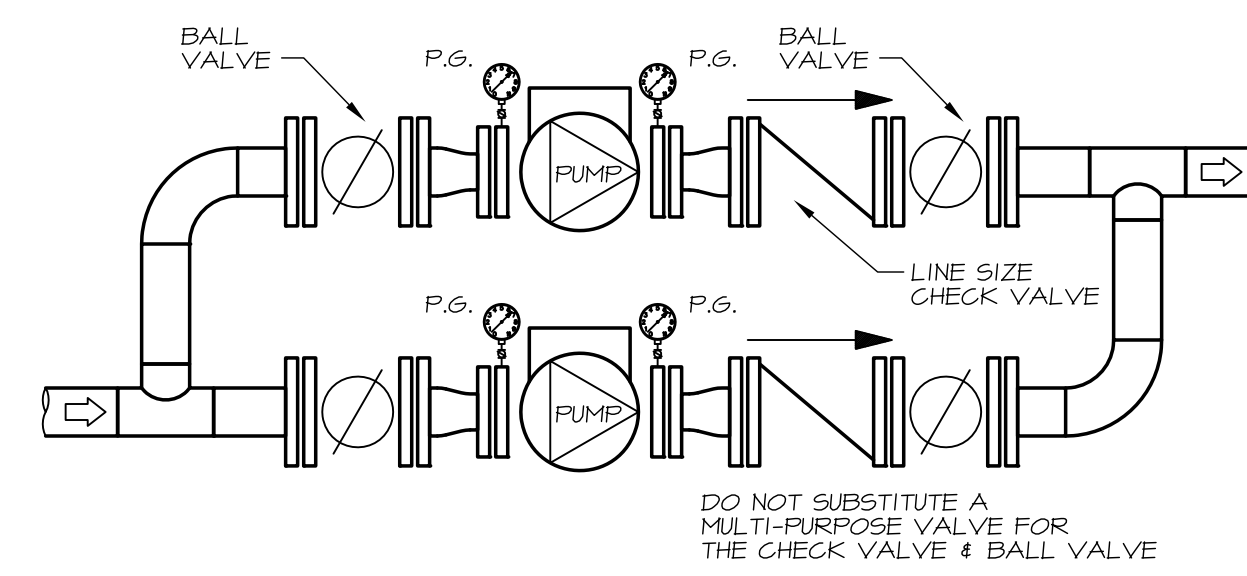
10 CIRCULATING PUMPS PIPING NO SCALE
