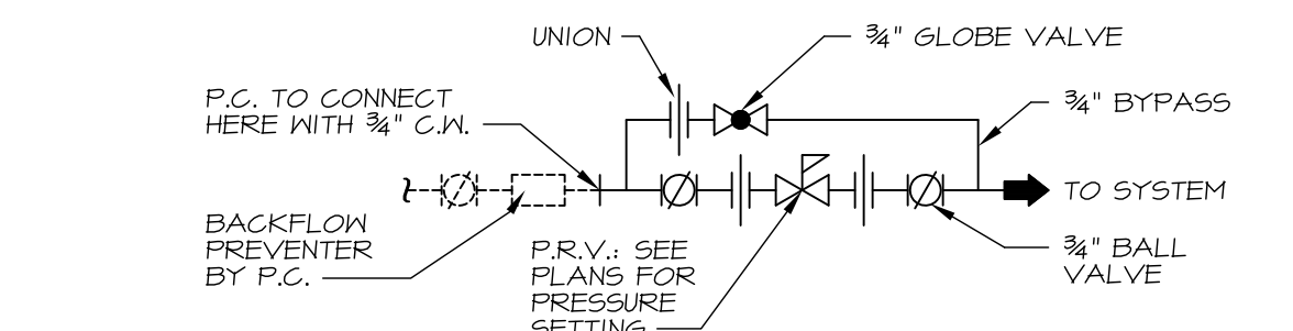
9 HEATING SYSTEM WATER MAKE-UP DETAIL NO SCALE
