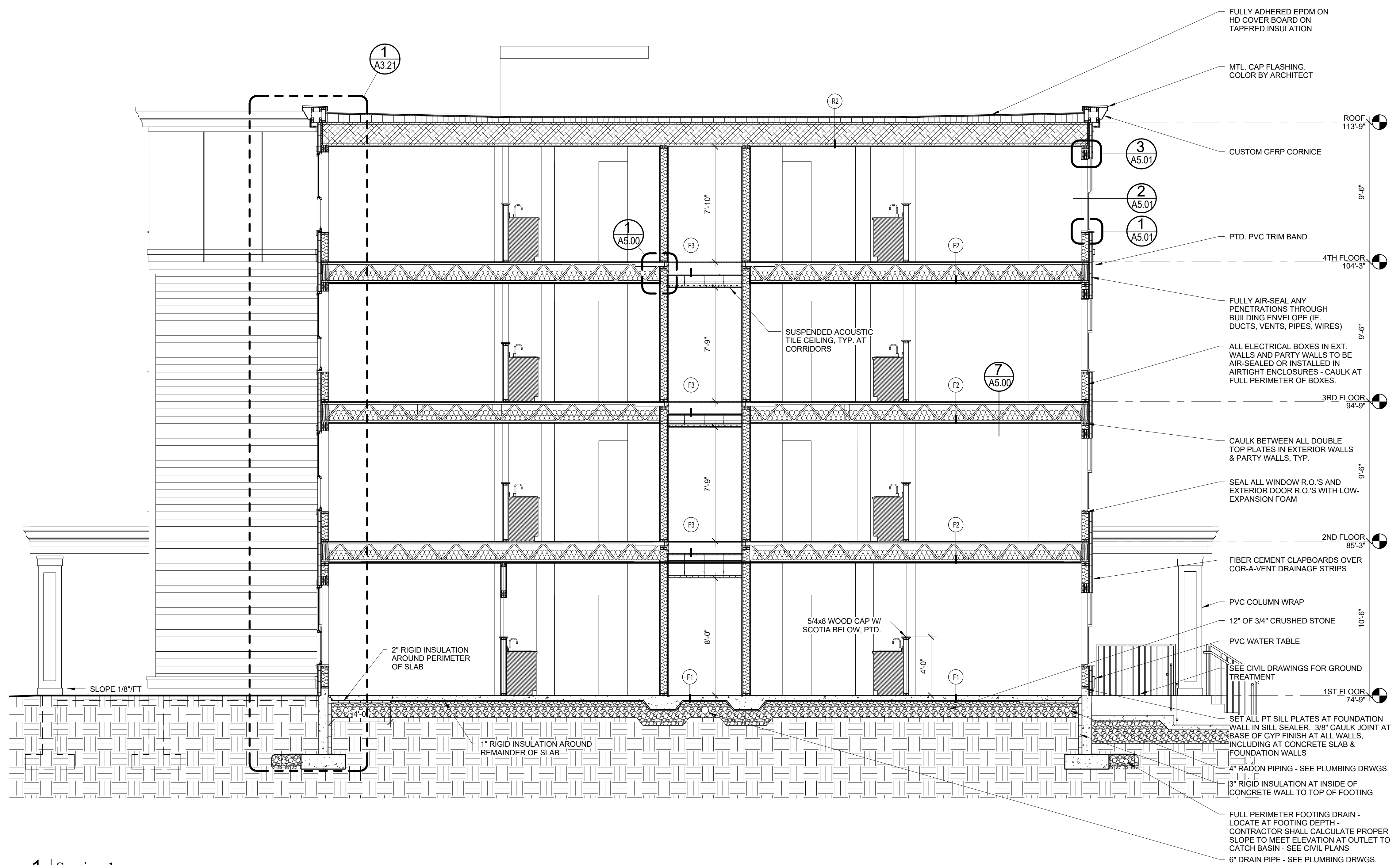
1 Section 1 1/4" = 1'-0"
