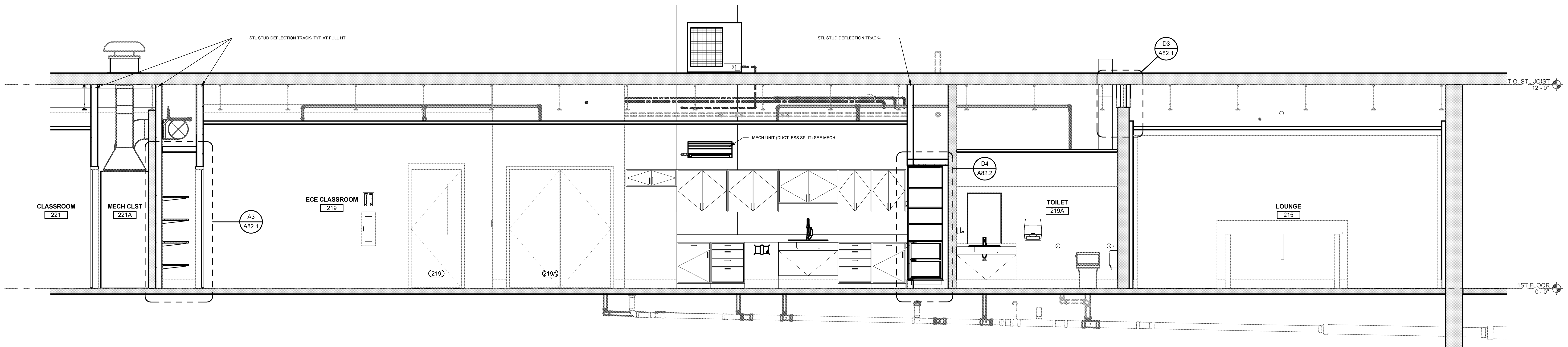
B1 BUILDING SECTION B1 SCALE: 3/8" = 1'-0"
