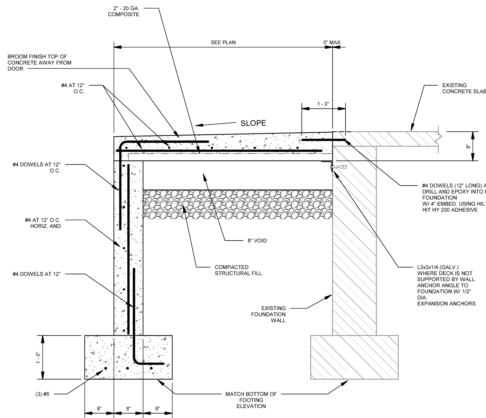
C2 TYP. ENTRANCE SLAB DETAIL SCALE: 3/4" = 1'-0"
