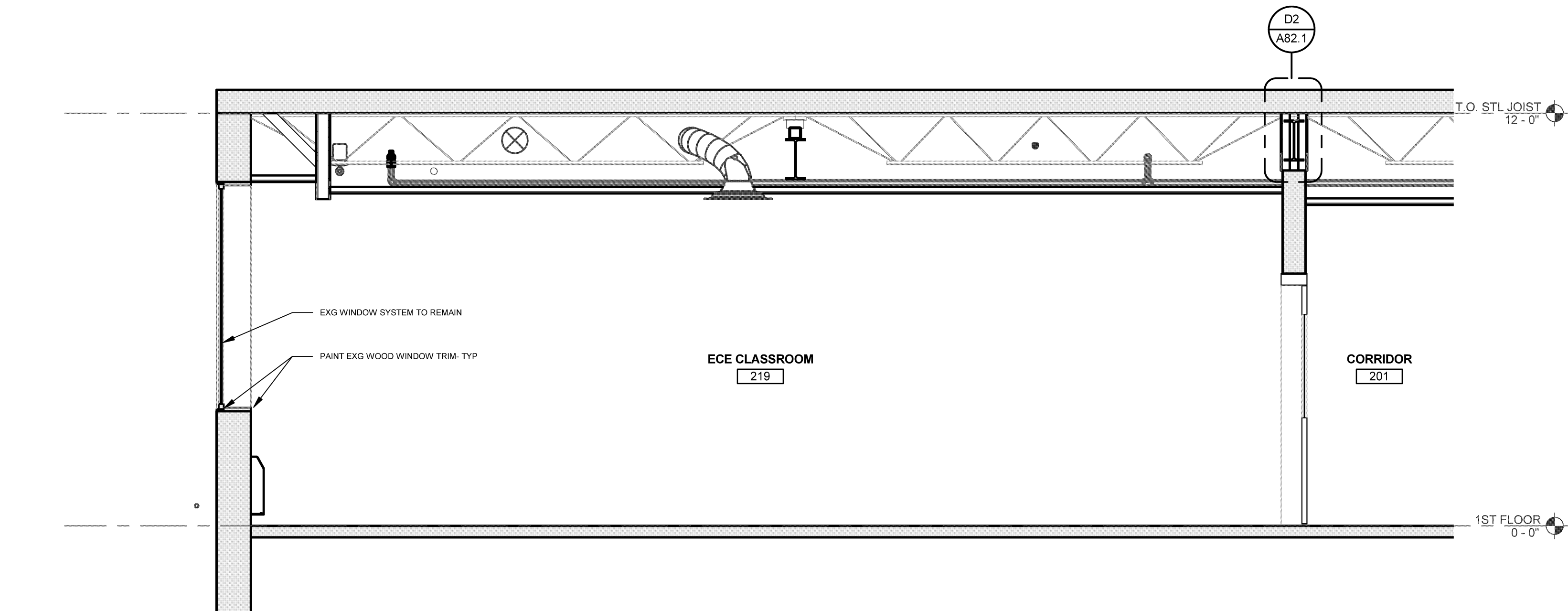
C1 BUILDING SECTION C1 SCALE: 3/8" = 1'-0"
